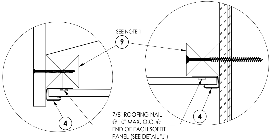
DETAIL "E"
