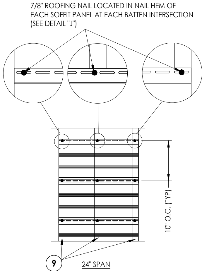
DETAIL "E"
